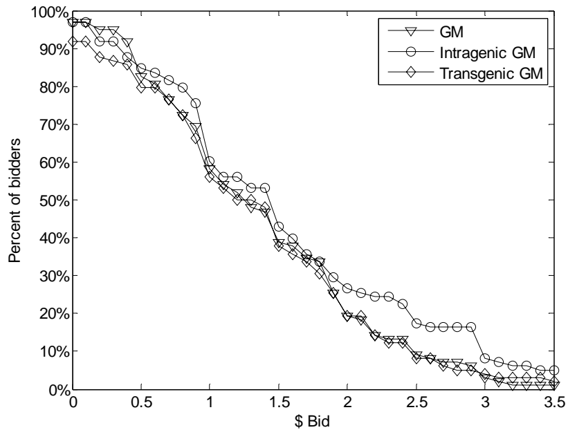
Figure 3.4 Inverse CDF of Bid Prices for Broccoli With PECA
